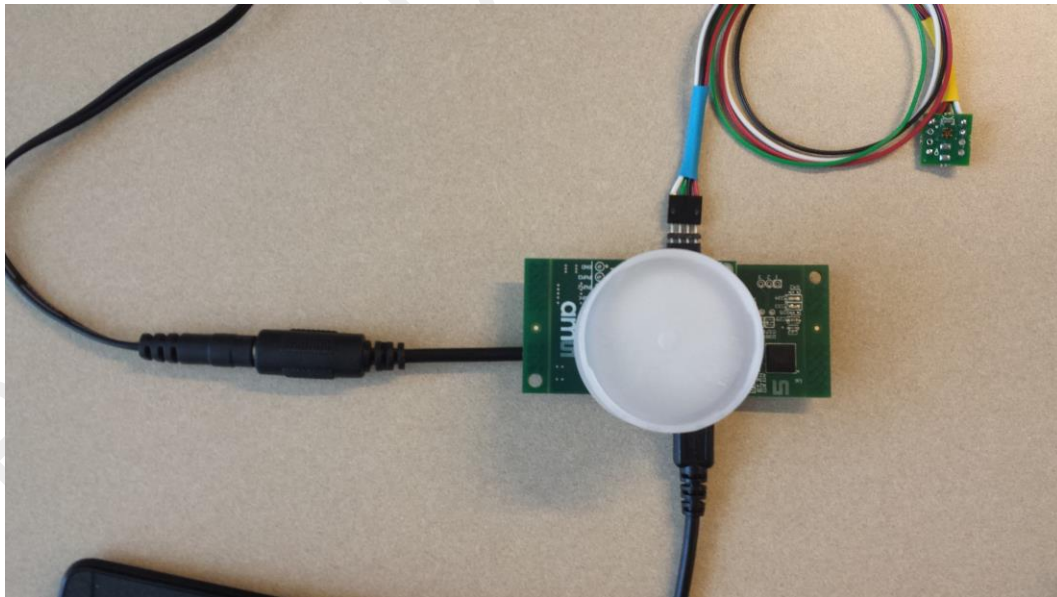
Figure 2. AS7221 SLIK & AS4531 – Connected to PC & DC Power
