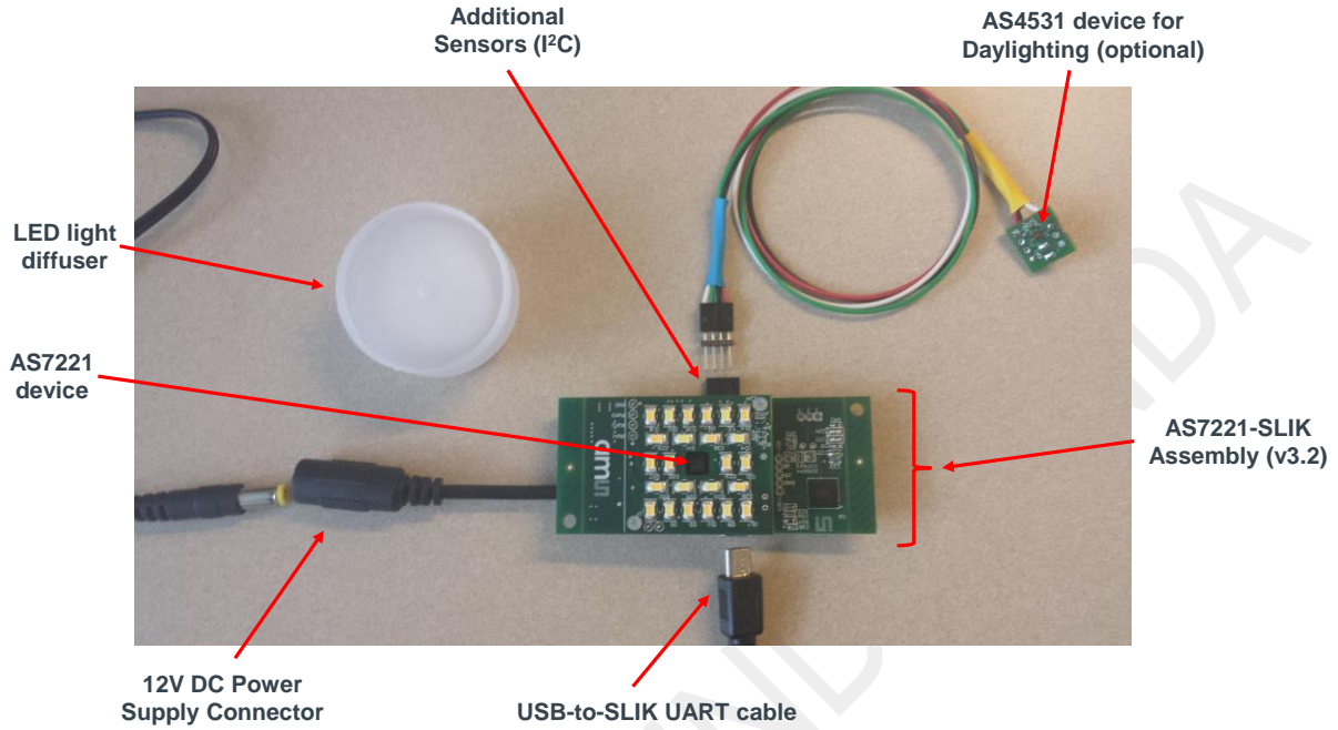
Figure 1. AS7221 SLIK & AS4531 – Disconnected from PC & Power
