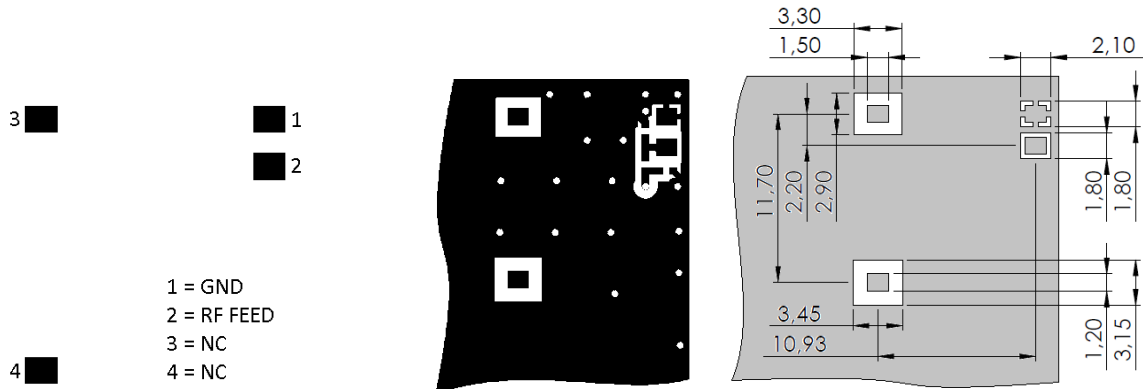
Pin configuration
