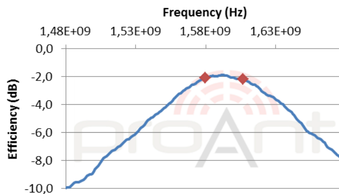
Total efficiency
