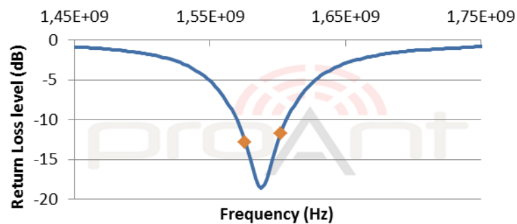
Return Loss
