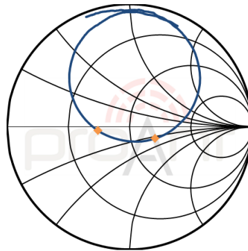
Smith chart
