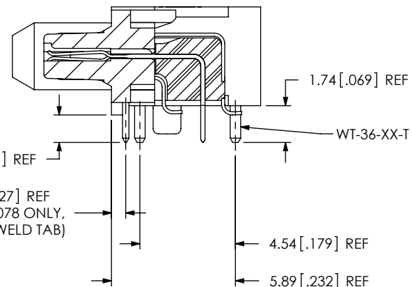
SECTION "J"-"J"
