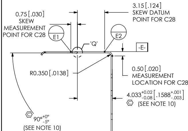
IN-PROCESS 6 (FORM 1 CONTACT T-1M52-04-X) (LEFT SIDE SHOWN)
