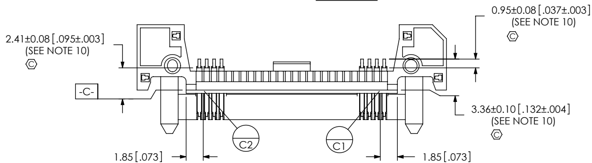
INSPECTION FOR IN-PROCESS 3 & 4 (CARRIER NOT SHOWN FOR IN PROCESS 3 INSPECTIONS)
