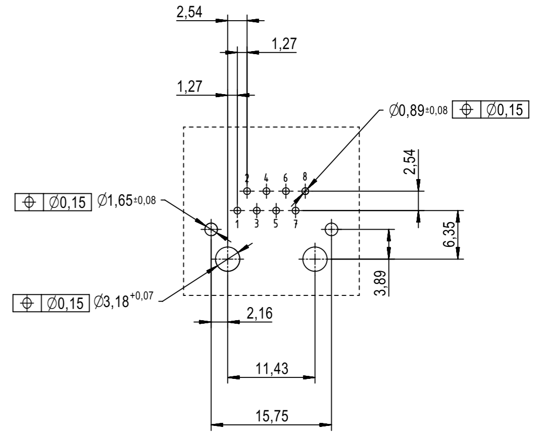
PC-Board layout view component side
