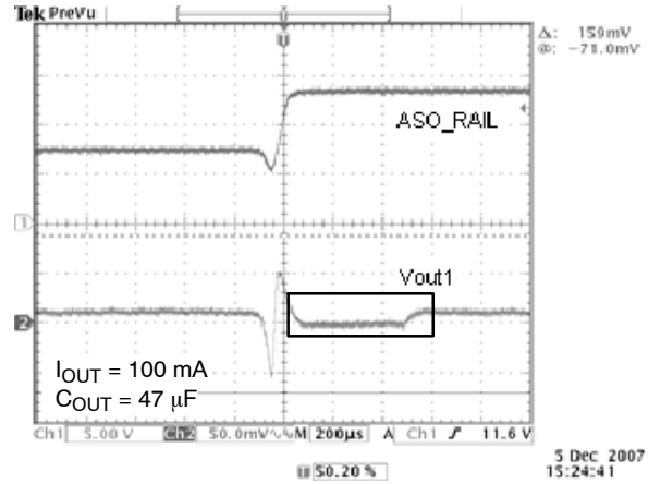
Figure 3. V_{\text{OUTX}} Response to ASO Switchover Event
