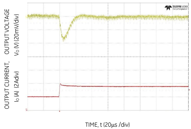
Figure 16. Transient Response to Dynamic Load Change from 50% to 100% at 12Vin, C out =5x47μF, C Tune =4.7nF, R Tune =300
