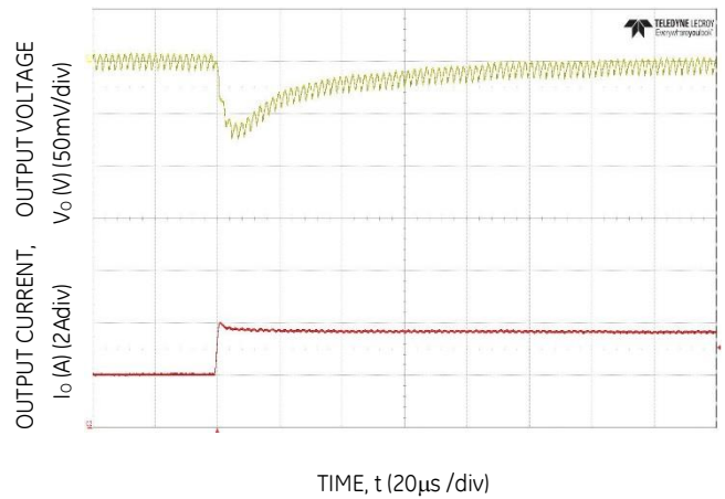
Figure 28 Transient Response to Dynamic Load Change from 50% to 100% at 12Vin, Cout=3x47uF, CTune=470pF, RTune=300
