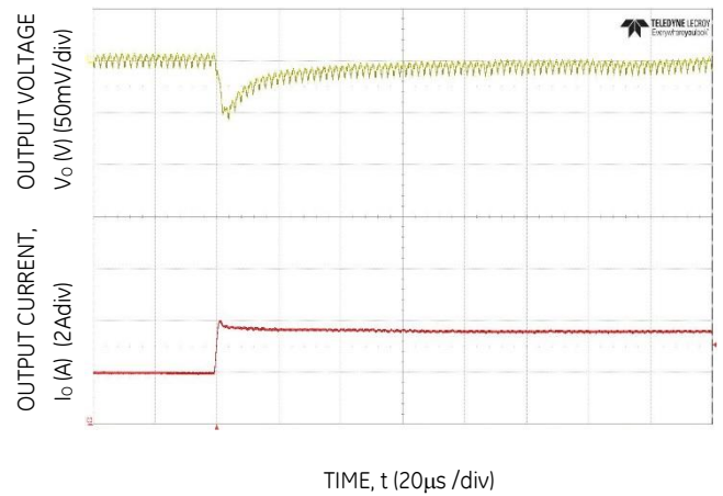
Figure 22. Transient Response to Dynamic Load Change from 50% to 100% at 12Vin, Cout=3x47uF, CTune=1.5nF, RTune=300
