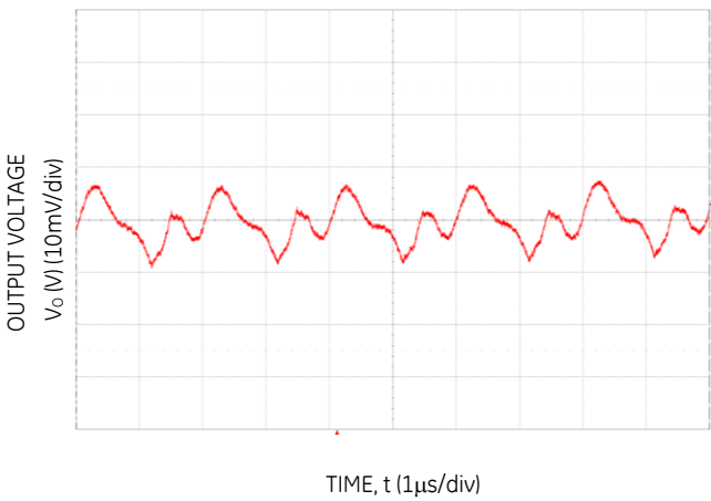
Figure 15. Typical output ripple and noise (C o =3X22μF ceramic, V IN = 12V, I o = I o,max ).
