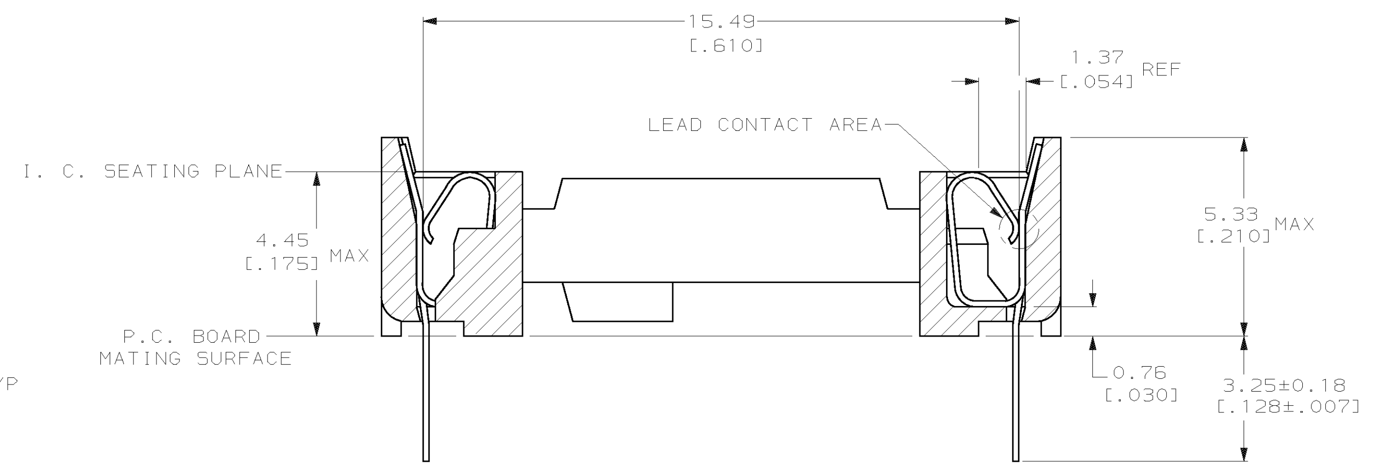
SECTION A-A ROTATED 90° CW SCALE 10:1
