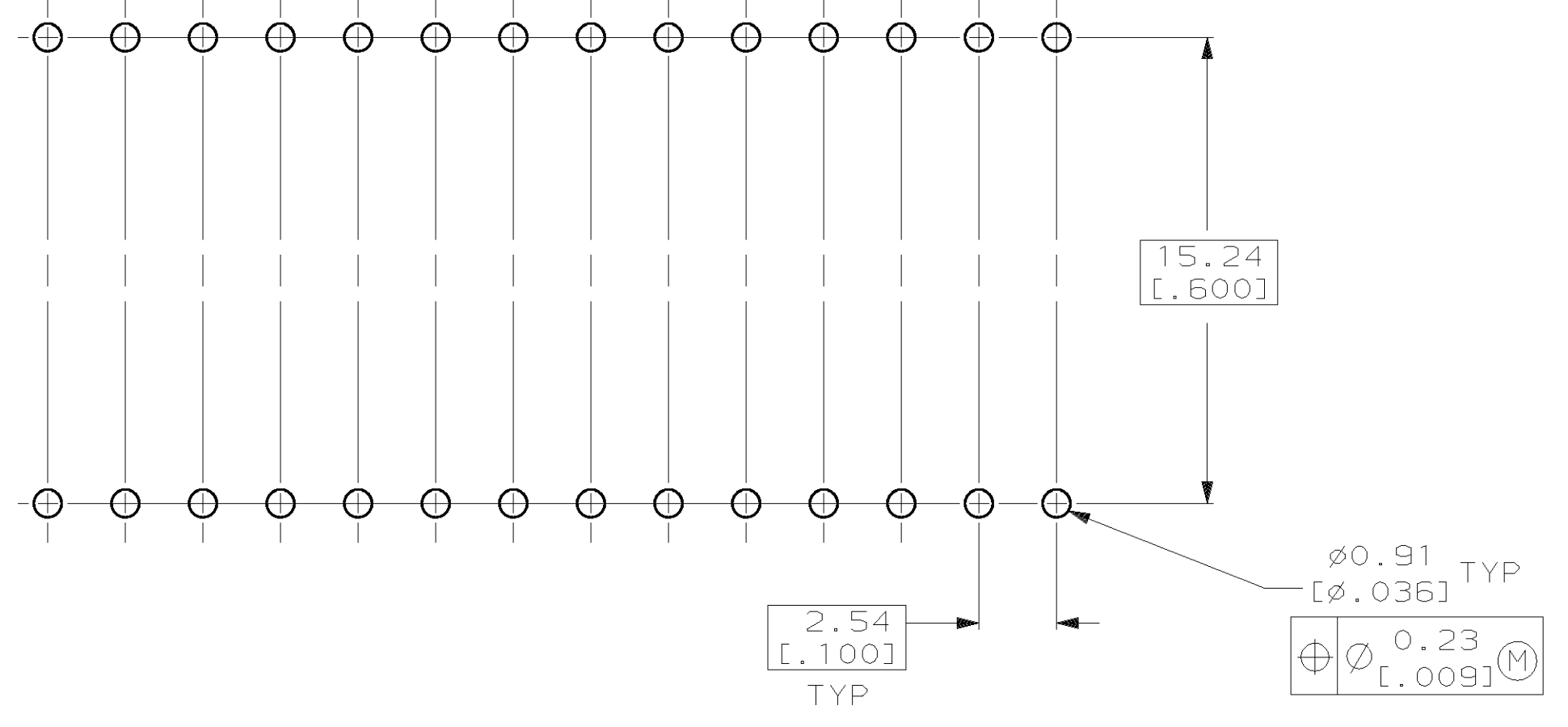
RECOMMENDED MOUNTING HOLE PATTERN
